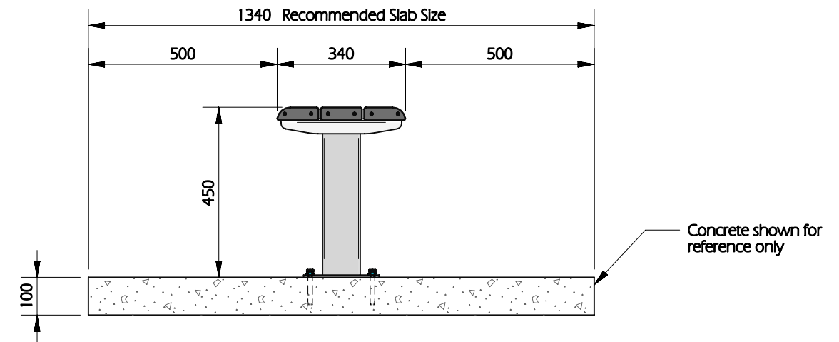
SIDE VIEW
