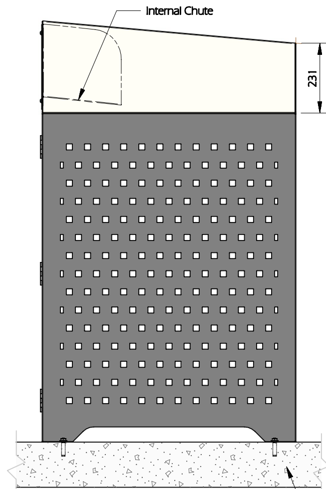
SIDE VIEW SCALE: NTS
