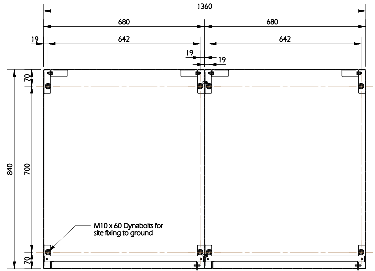
FOOTPRINT SECTION A-A SCALE 1:10
