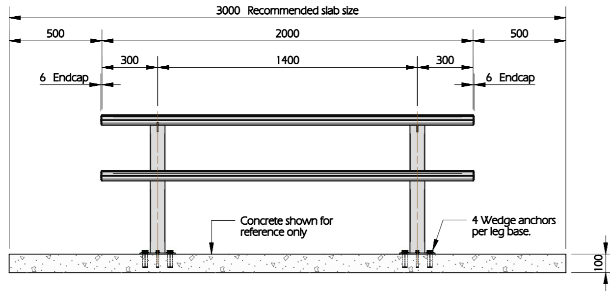
ELEVATION SCALE 1:20
